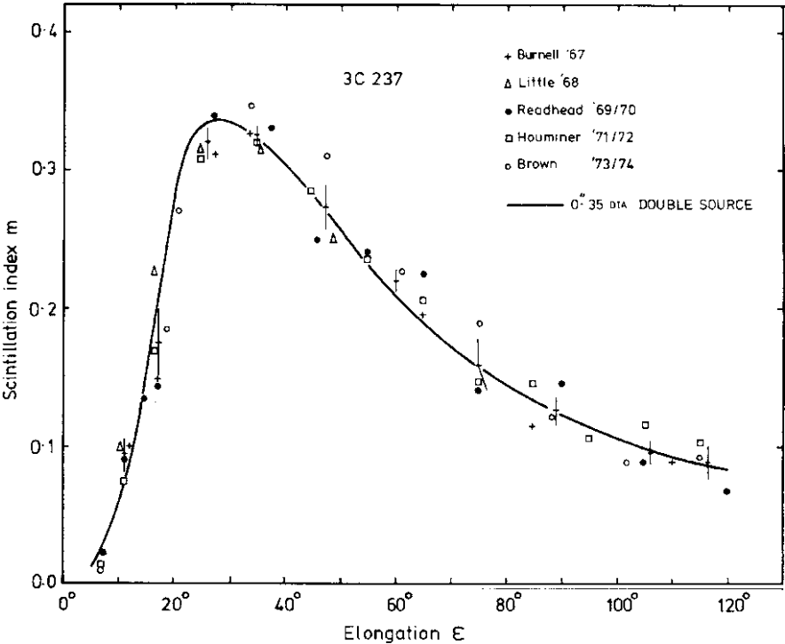
Fig. 6.2 Plot of scintillation S_{\text{rms}} (m) vs elongation \epsilon for the radio source 3C 237 [23]. Each value was obtained at different times of the year, when the source was at different elongations. The superimposed curve represents the RKH modeled fit through the data [23]
