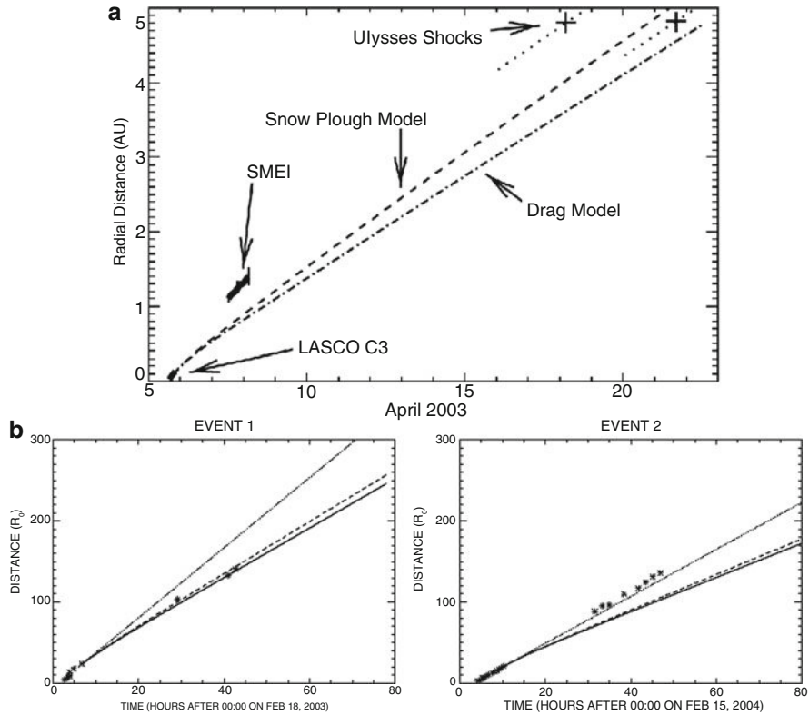
Fig. 9.2 Distance-time plots for three events studied comparing LASCO and SMEI data with the aerodynamic drag model. (a) Results from a single event in April 2003 reported by Tappin [43]. Labeled are the LASCO and SMEI height-time datasets, the arrival times of two shocks at Ulysses near 5 AU and the results from the Snow Plough and Aerodynamic Drag Models. (Reproduced with kind permission of Springer Science and Business Media). (b) Results from two events observed in February 2003 and 2004 (Howard et al. [20]). The crosses are the LASCO datasets, asterisks are SMEI datasets, and the heavy and dashed curves are for the Snow Plough and Aerodynamic Drag models respectively. Note that Event 1 (2003) shows an excellent fit with the drag models, while Event 2 requires an additional acceleration. This event is almost aligned with the constant speed line (dotted), which shows the trajectory of the CME if it were to retain the same speed it had when leaving the LASCO field of view. (Reproduced by permission of the AAS)
