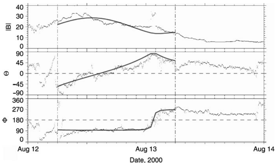
Fig. 7.17 Magnetic field plot of the magnetic cloud observed in August 2000 with the WIND spacecraft. The top plot represents the total magnetic field while the second and third plots are the spherical coordinates ( \Theta , \Phi ) of the measured field. The signature of the cloud is represented by the smooth rotation of the magnetic field [48]. The grey overlaid curve is the force-free solution determined by Leamon et al. [48]
