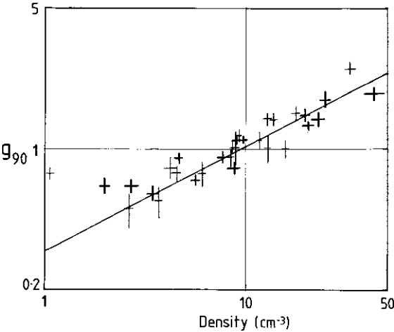
Fig. 6.3 Plot of the relative scintillation index g vs density N_e for a number of events where IPS transients were clearly associated with an in-situ ICME. Note the power-law relationship between the two (linear in this log-log plot), which can be used to relate g and N_e for future IPS measurements [28]. (Reprinted with permission from Elsevier)
