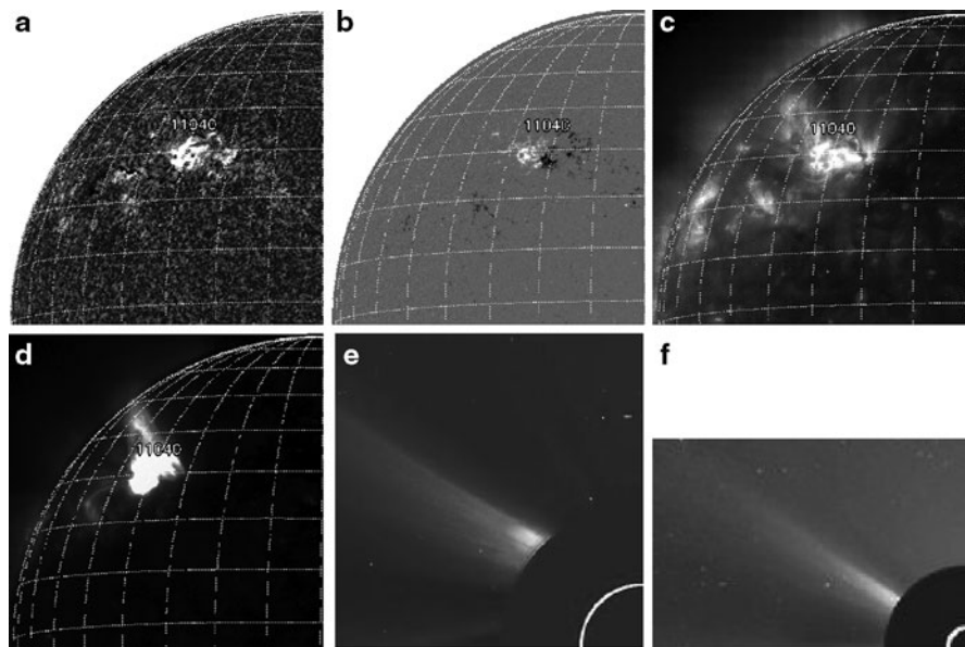
Fig. 7.3 Active region AR11040 (1040) observed in January 2010. It is shown here on 10 January observed by (a) H\alpha (Kanzelhoehe), (b) magnetogram (SOHO/MDI, and (c) EUV (SOHO/EIT 195 Å). (d) The x-ray (Hinode/XRT) image was obtained on 9 January and the SOHO/LASCO (e) C2 and (f) C3 coronagraph images were obtained on 8 January, when the active region was near the northeast limb. Data supplied courtesy of Solarmonitor.org (Trinity College, Dublin)
