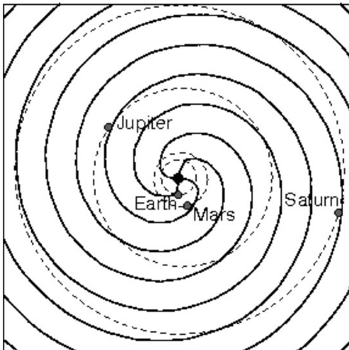
Fig. 9.7 Diagram of the Parker spirals (heavy curves) in the ecliptic plane similar to that shown in Fig. 9.1, but extended out to 10 AU. The orbits of the Earth, Mars Jupiter and Saturn are shown (dashed ellipses), along with their locations at 1 January 2010
