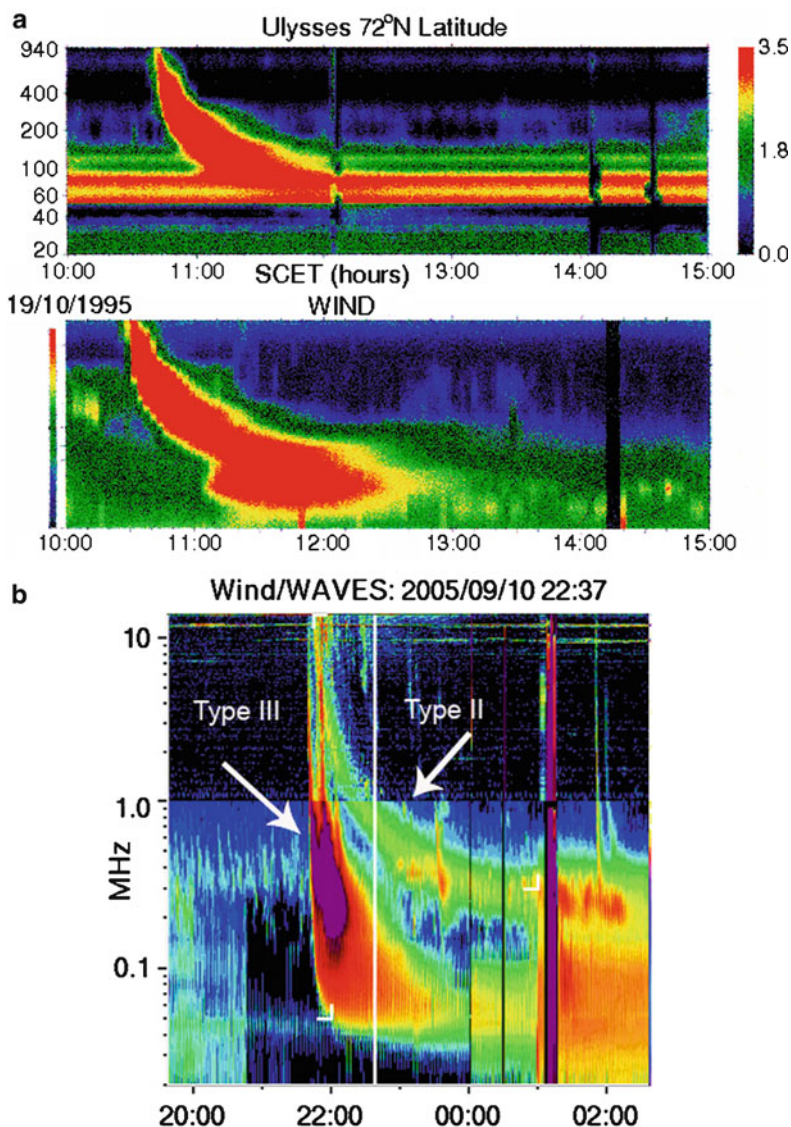
Fig. 7.18 (a) Type II burst observed with Ulysses and WIND [66]. (b) Dynamic spectrum of a Type II and accompanying Type III radio burst observed with the WIND /Waves radio telescope on 10 September 2005 [27]. (Reproduced by permission of the AAS)
