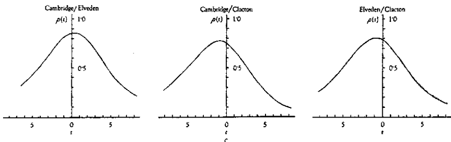
Fig. 6.5 Cross-correlograms from IPS observations on 9 May 1966, observed with a network of observatories in the UK. Note the time difference ( \tau -axis) between each [9]. (Reprinted by permission from Macmillan Publishers Ltd: Nature [9], Copyright 1967)
