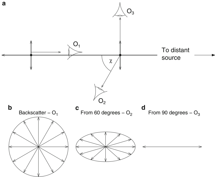
Fig. 4.1 Schematic demonstrating how the angular variation in Thomson scattering arises (a) the conceptual set up, the scattering angle \chi is shown for the oblique observer ( O_2 ), (b–d) the scattered electric vectors as seen by observers at O_1 at \chi = 180^\circ , O_2 at \chi = 60^\circ and O_3 at \chi = 90^\circ respectively [2]. (Reproduced with kind permission of Springer Science and Business Media)
