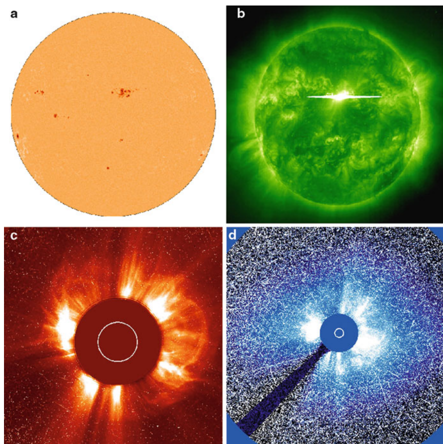
Fig. 7.6 Images of the famous “Bastille Day” flare on 14 July 2000. The solar disk during the flare is shown in (a) Dopplergram ( SOHO /MDI (taken 20:48 UT), (b) EUV ( SOHO /EIT), and white light coronagraphs (c) LASCO/C2 (at 10:54 UT) and (d) LASCO C3 (at 11:42 UT). The “snowstorm” appearance in C3 is due to energetic particles impacting the camera (Images courtesy of NASA)
