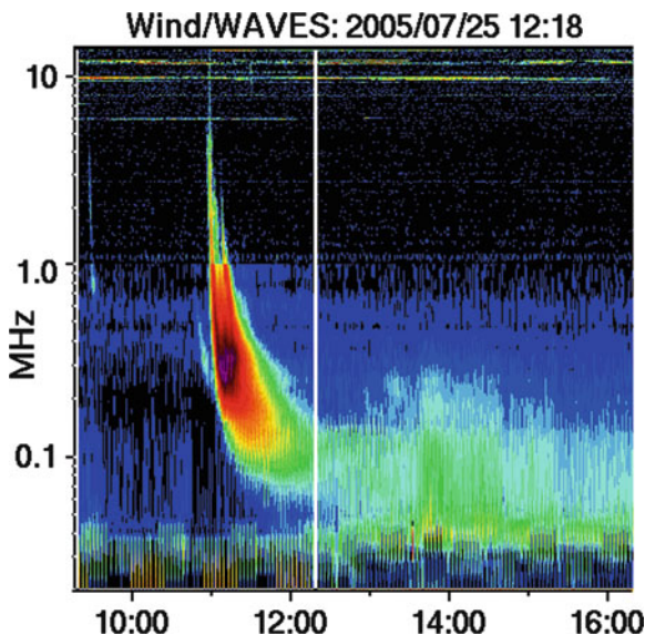
Fig. 7.12 Dynamic spectrum (with the log of frequency) of a Type III radio burst observed with the WIND/Waves radio telescope on 25 July 2005. The burst lasted for over 2 h and spanned several orders of frequency magnitude [27]. (Reproduced by permission of the AAS)
