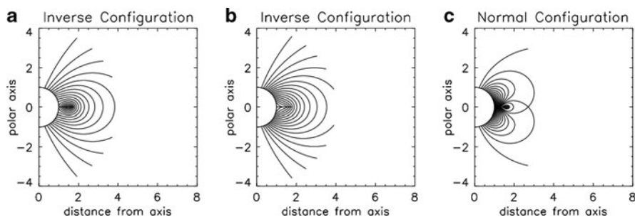
Fig. 8.4 Modeled magnetic field configurations for the two types of prominences, governed by the Mass Loading model, with the prominence sheet in the equatorial plane [15]. (a) An inverse prominence with the base normal flux distribution in the form of a dipole potential field. The resulting Lorentz force arises from the tension force being outward near the base but inward near the rim. (b) Inverse prominence with the dipole field increased so that the Lorentz force is radially inward along the prominence sheet. (c) Normal prominence with the dipole field reduced to allow closed field lines to form over the current. (Reproduced by permission of the AAS)
