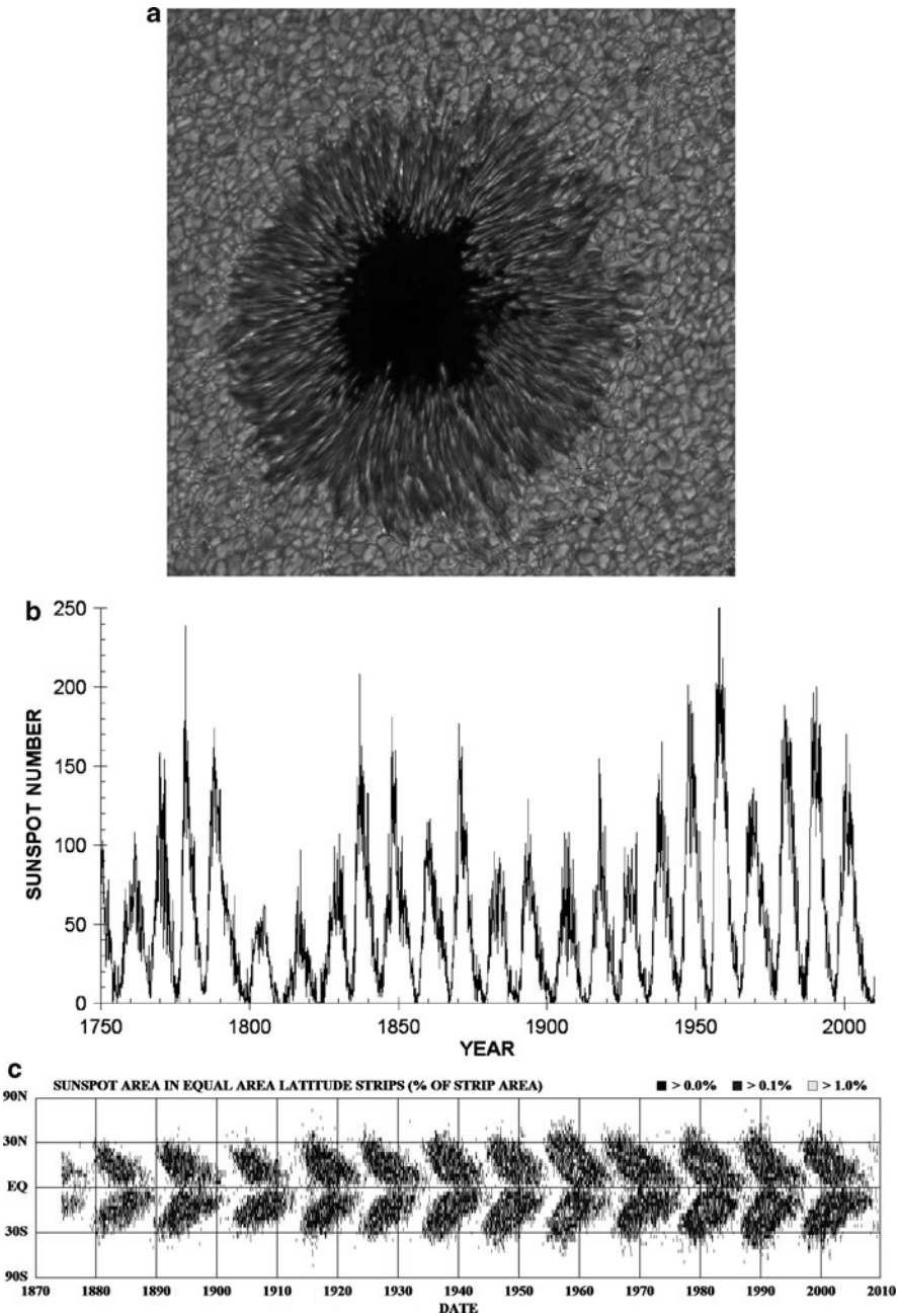
Fig. 7.5 (a) An image of a sunspot taken from the Big Bear Solar Observatory on 27 August 1999 [14]. (Reproduced with kind permission of Springer Science and Business Media). (b) and (c) trends across the solar cycle for sunspot activity. (b) Sunspot number per month as a function of time from 1750 to 2010. (c) Sunspot location (heliographic latitude) and area against time across 12 solar cycles (12–23) from 1875 to 2010 (Available courtesy of NASA)
